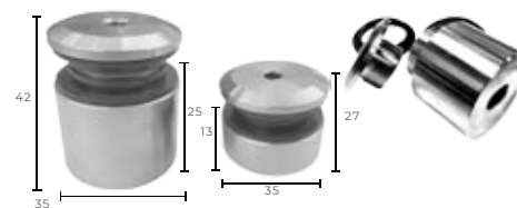
Item No: G-C576 品名：玻璃与墙体固定件 Name: Adjustable single point fixing
