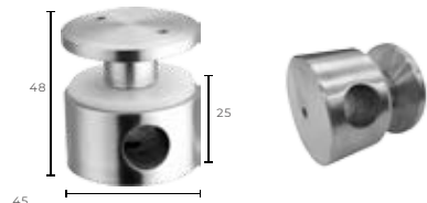
Item No: G-C580 品名：玻璃与墙体固定件 Name: Adjustable single point fixing
