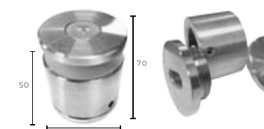
Item No: G-C572 品名：玻璃与墙体固定件 Name: Adjustable single point fixing
