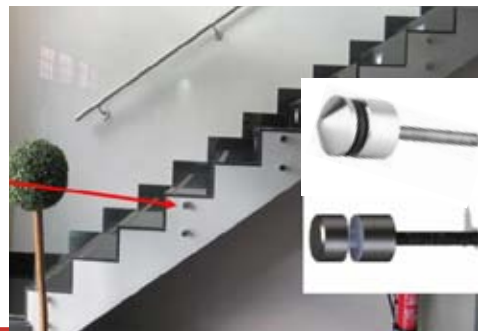
Item No: G-C583 品名：玻璃与墙体固定件 Name: Adjustable single point fixing
