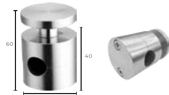
Item No: G-C581 品名：玻璃与墙体固定件 Name: Adjustable single point fixing
