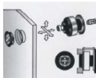
Item No: G-C582 品名：玻璃与墙体固定件 Name: Adjustable single point fixing
